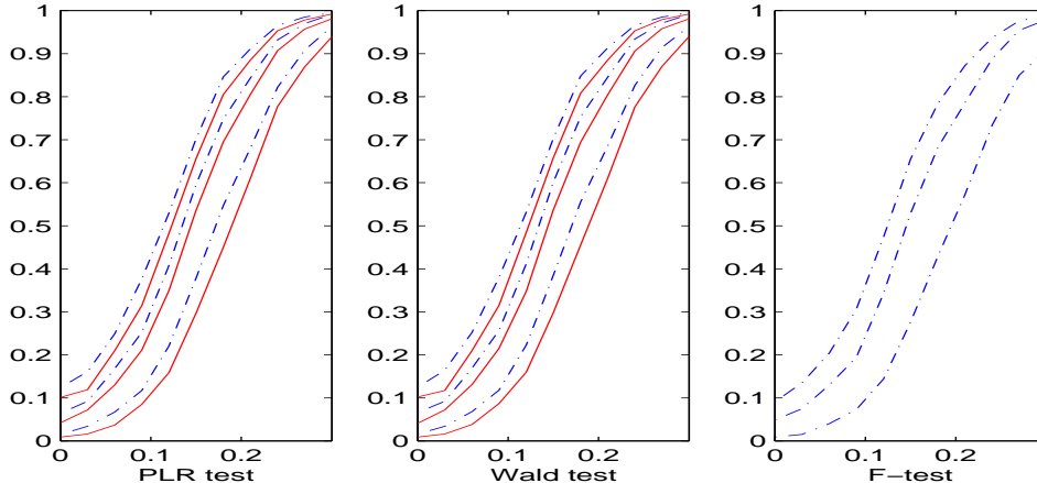
Figure 2: The simulated power functions for Case I with h = .625 . The critical values are computed by \chi_2^2 -approximation (dash-dot lines) and the conditional bootstrap method (solid lines). (a) PLR test, (b) Wald test, (c) F-test.
