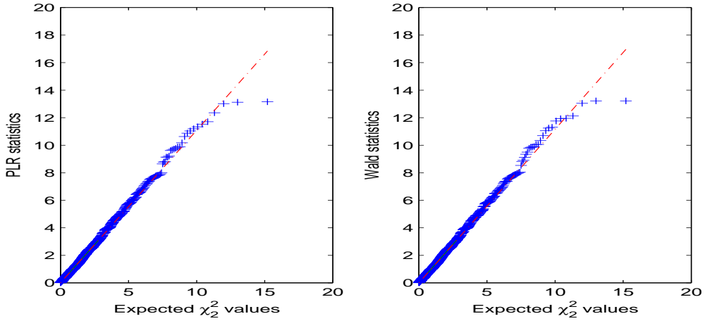
Figure 3: The Q-Q plots, h = .25 . (a) PLR statistics. (b) Wald statistics.
