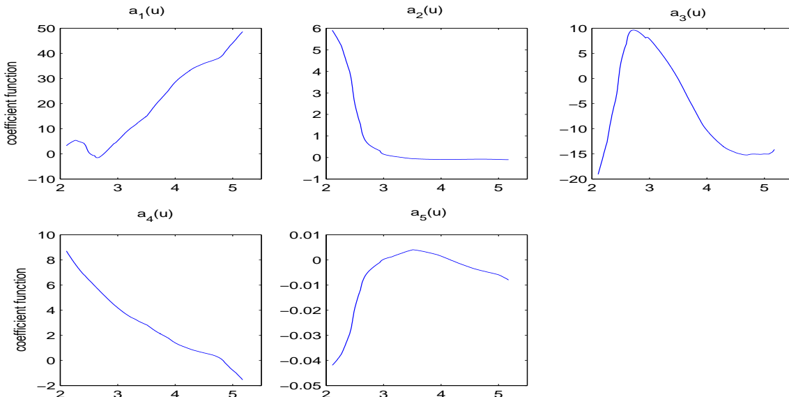
Figure 5: The estimated coefficient functions.
