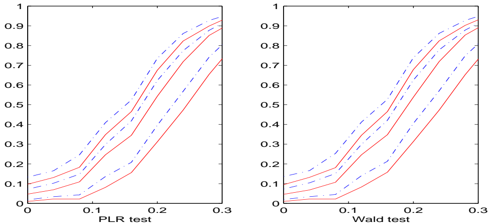
Figure 4: The simulated power functions with h = .625 . The critical values are computed by \chi^2 -approximation (dash-dot lines) and the conditional bootstrap method (solid lines). (a) PLR test, (b) Wald test.
