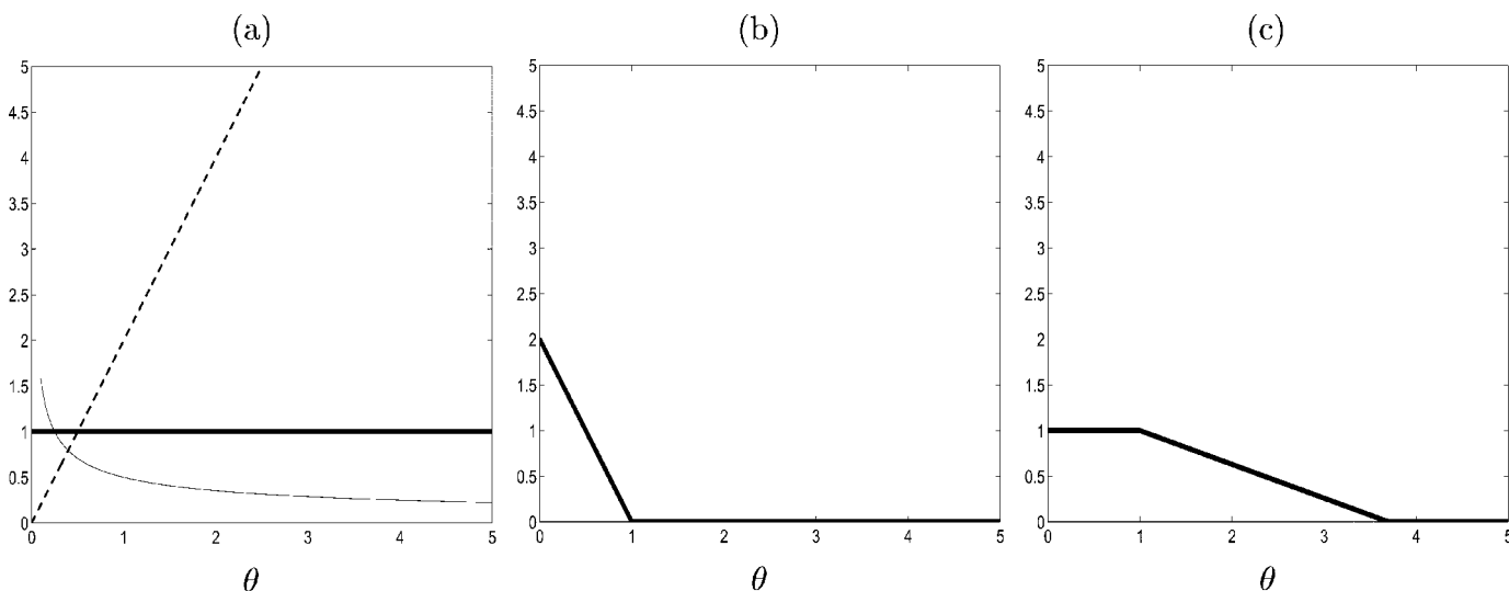
Figure 4. Plot of p_\lambda(\theta) Functions Over \theta > 0 (a) for L_q Penalties, (b) the Hard Thresholding Penalty, and (c) the SCAD Penalty. In (a), the heavy line corresponds to L_1 , the dash-dot line corresponds to L_5 , and the thin line corresponds to L_2 penalties.
